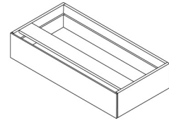
Brix Mid Box 100 BRX100M L 100cm D 50cm H 20cm / L 39" D 19 1/2" H 7 3/4"
